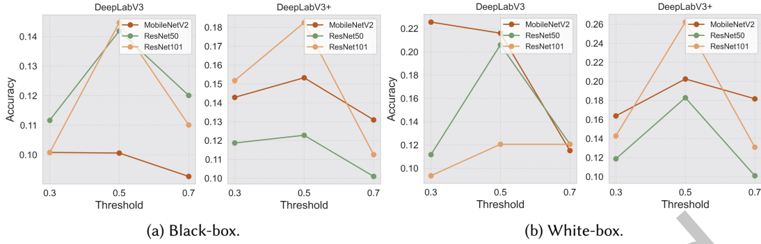
Fig. 9. The attribute inference attack accuracy of the pruned models among the three pruning thresholds (0.3, 0.5, and 0.7).
