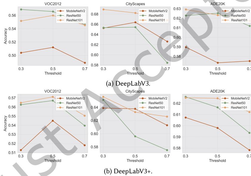
Fig. 11. The model inversion attack accuracy of the pruned models.
