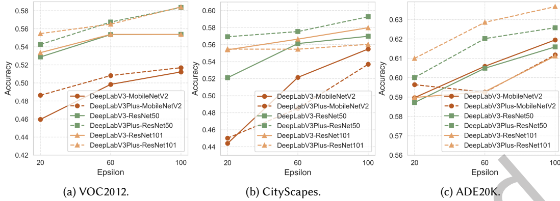
Fig. 10. The accuracy of model inversion attacks under different \epsilon in DP. The attack performance improves with the increase of \epsilon .
