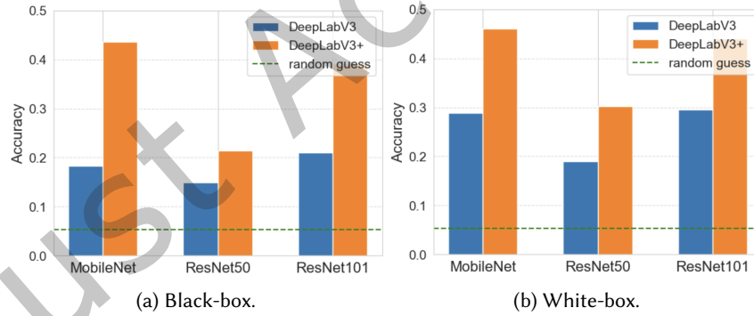
Fig. 8. The attribute inference attack accuracy in black-box and white-box settings. The random guessing is the inverse of the total number of cities.
