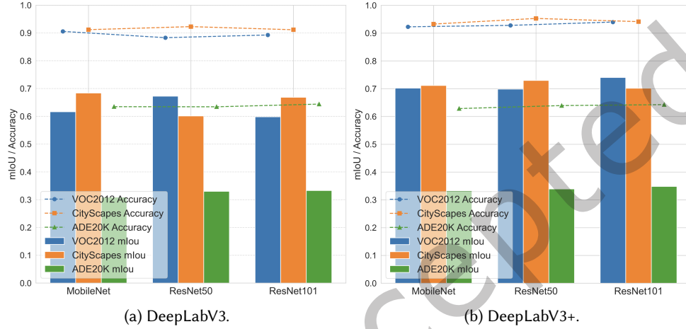
Fig. 4. The mIoU and pixel accuracy of shadow models using three backbones (MobileNetV2, ResNet50, and ResNet101) across different datasets for both DeepLabV3 and DeepLabV3+.
