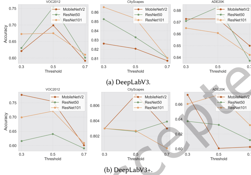
Fig. 7. The ablation study of the membership inference attack accuracy of the pruned models among the three pruning thresholds.
