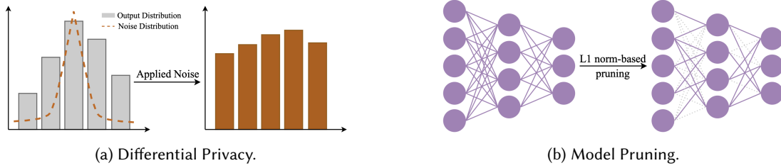
Fig. 3. Defense mechanism principles. In differential privacy, by introducing the Laplace noise distribution into the original distribution, the output distribution is smoothed, making it difficult to infer the presence of any individual data point. In model pruning, the less important weights are removed to reduce the model's complexity and mitigate overfitting, which helps to privacy-preserving.
