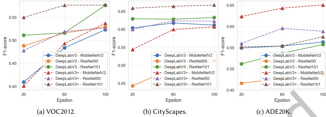
Fig. 6. F1-score of membership inference attacks under different \epsilon in DP. The attack performance improves with the increase of \epsilon .
