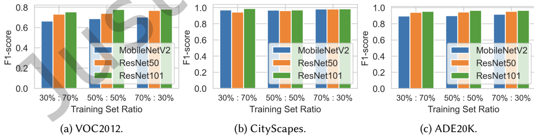
Fig. 5. The F1-score comparison of membership inference attacks across three backbones in DeepLabV3, exploring the impact of different ratios of shadow model training sets and victim model training sets on the attack performance.
