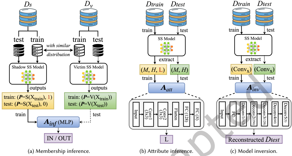
Fig. 2. The structure of membership inference, attribute inference, and model inversion attacks. In membership inference, \mathcal{A}_{inf} is the membership inference attack model, \mathbf{P} represents the combined mean and standard posterior probability from the model, and 0 and 1 are the corresponding membership labels. In attribute inference, \mathcal{A}_{att} is the attribute inference attack model, \mathbf{M} and \mathbf{H} denote the image mask and color histograms, respectively, and the L is the city label. In model inversion, \mathcal{A}_{inv} is the model inversion model, Conv_x represents the features from the intermediate convolutional layer x .
