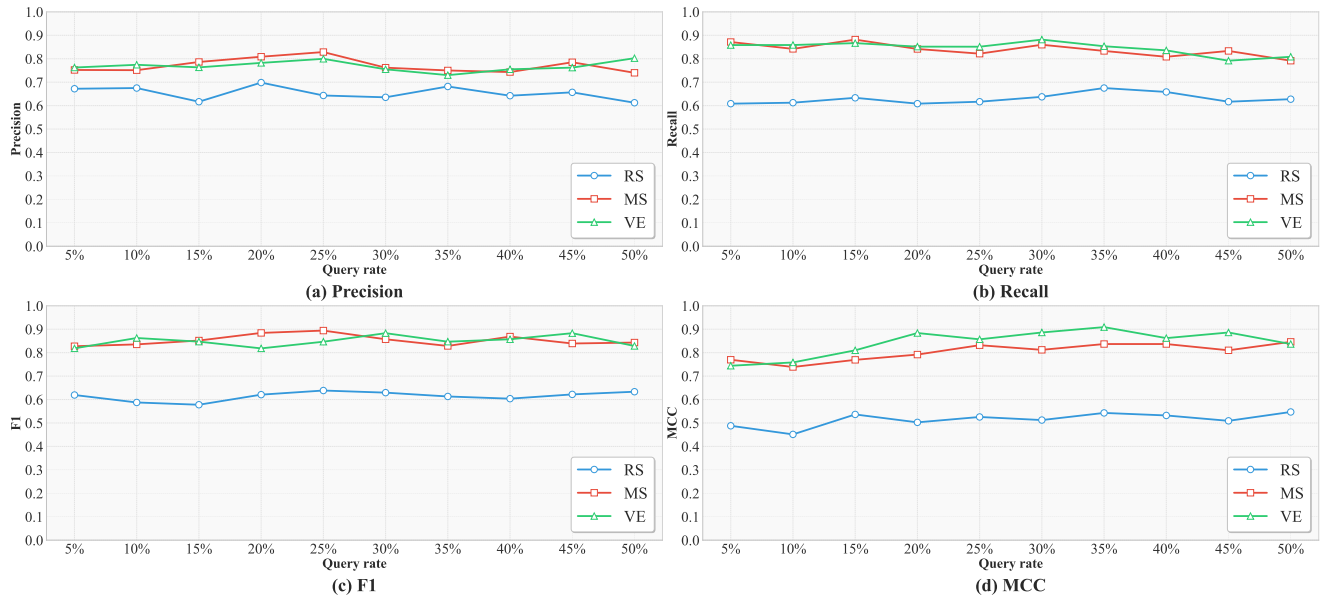
Fig. 11. The performance of code smell detection models with VE, MS, and RS query strategies for Long Method detection (query rate: 5%–50%).
