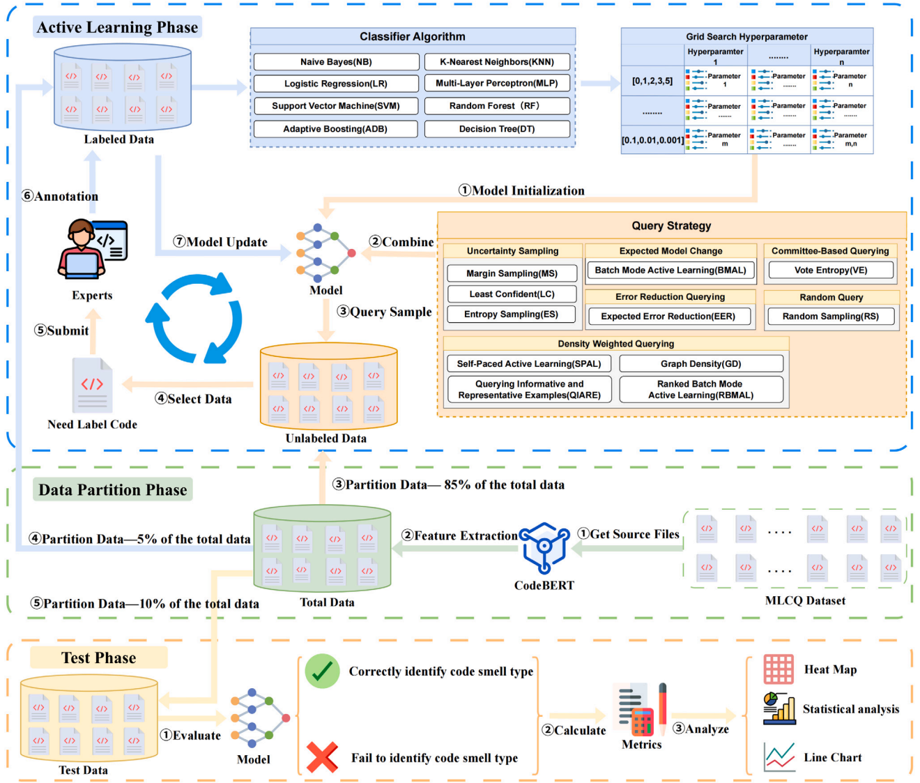
Fig. 3. The overall experimental process of code smell detection based on active learning.
