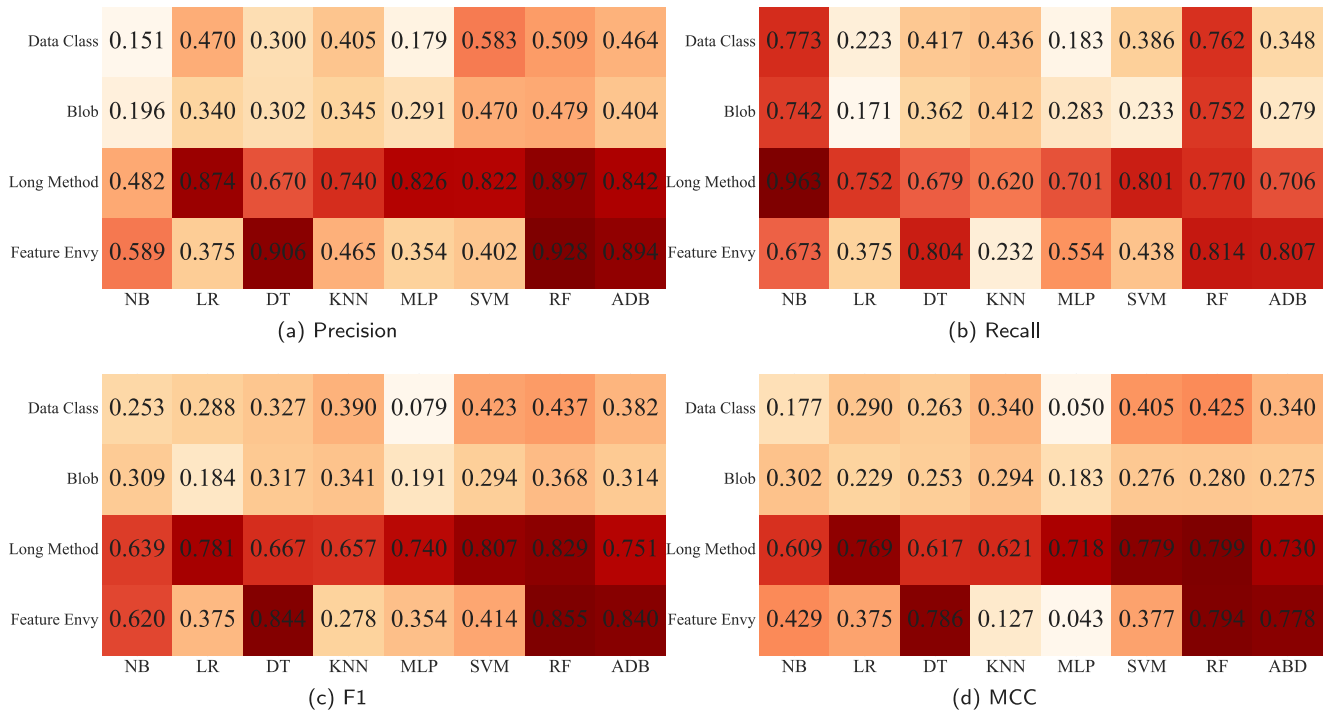
Fig. 7. The average precision, recall, F1-score, and MCC values of the 8 classifiers across code smell types and query strategies.
