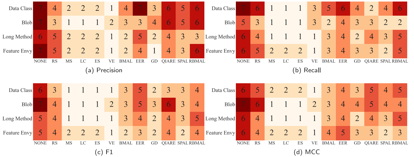
Fig. 6. The Scott-Knott ESD rankings of the 11 query strategies across code smell types and classifiers in terms of precision, recall, F1-score, and MCC.
