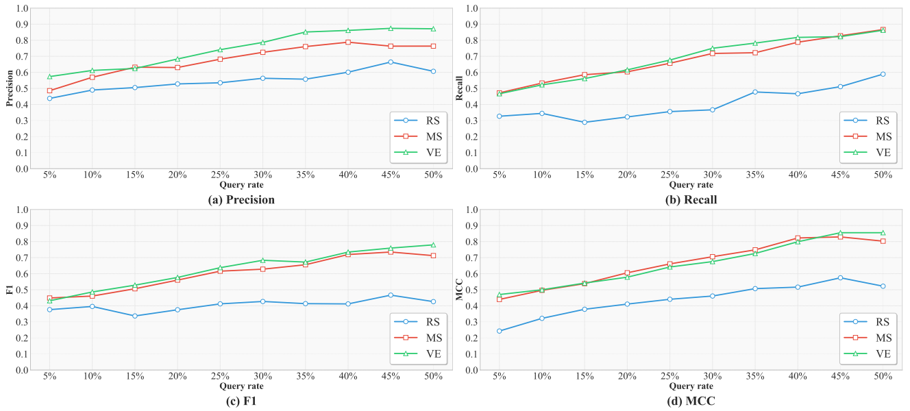
Fig. 9. The performance of code smell detection models with VE, MS, and RS query strategies for Data Class detection (query rate: 5%–50%).
