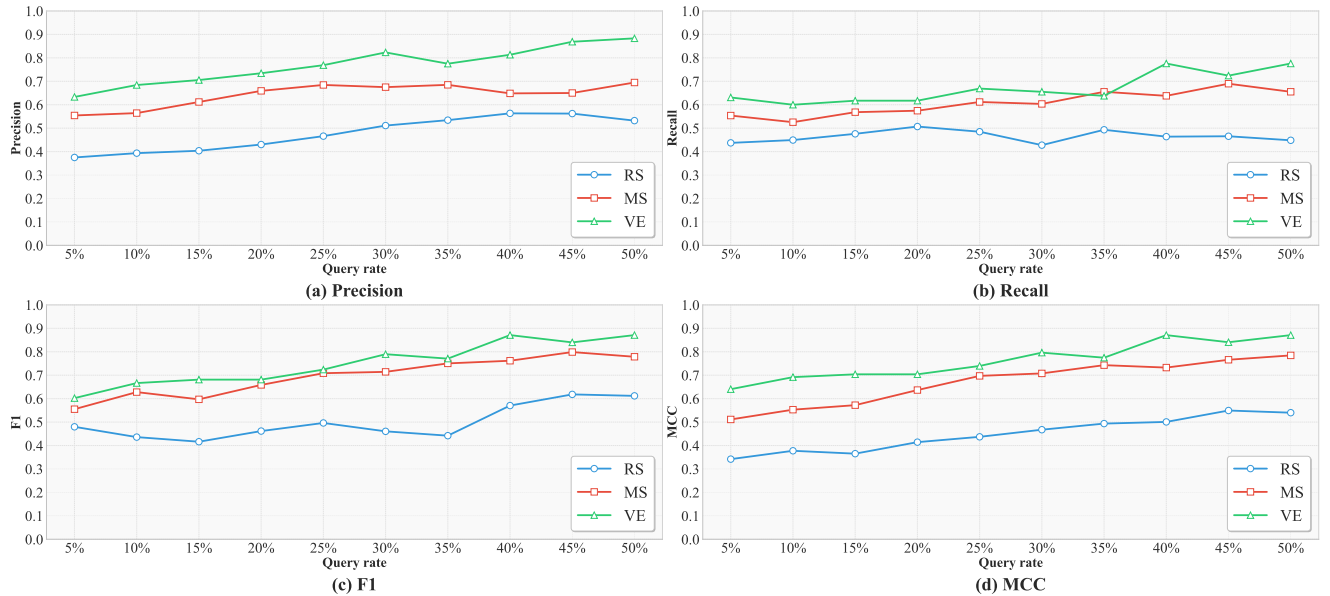
Fig. 12. The performance of code smell detection models with VE, MS, and RS query strategies for Feature Env detection (query rate: 5%–50%).
