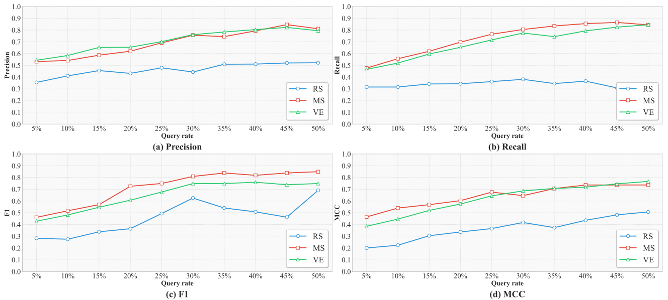
Fig. 10. The performance of code smell detection models with VE, MS, and RS query strategies for Blob detection (query rate: 5%–50%).
