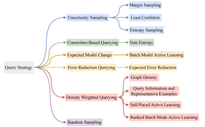
Fig. 2. The eleven query strategies investigated in our study.
