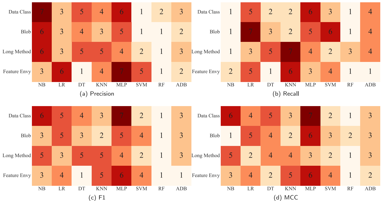
Fig. 8. The Scott-Knott ESD rankings of the 8 classifiers across code smell types and query strategies in terms of precision, recall, F1-score, and MCC.
