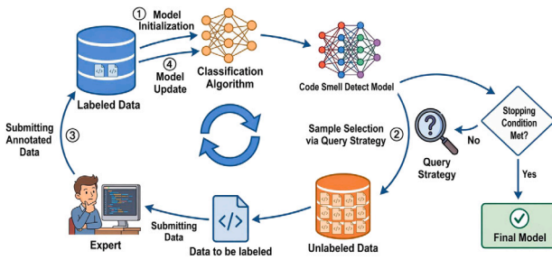
Fig. 1. The overview of the active learning workflow for code smell detection.
