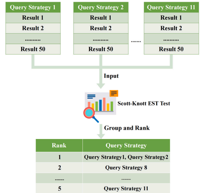
Fig. 4. The example of the Scott-Knott ESD test.
