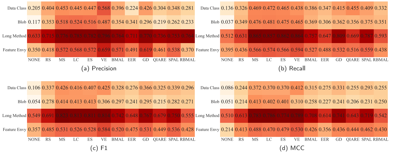
Fig. 5. The average precision, recall, F1-score, and MCC values of the 11 query strategies across code smell types and classifiers.
