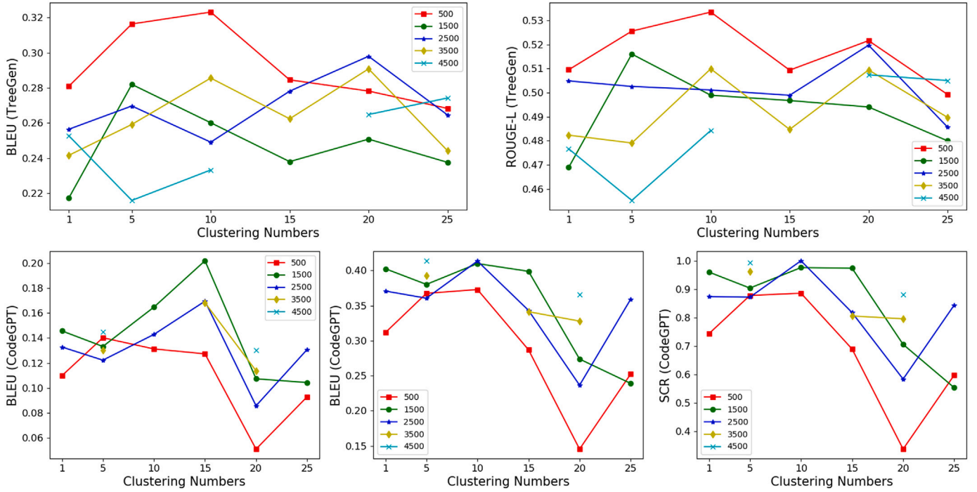
Fig. 5. The influence of clustering numbers on MetaCoder.
