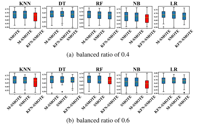
Fig. 12. The Scott-Knott ESD test ranking of the performance of SMOTE, M-SMOTE, and KFN-SMOTE in terms of AUC on the five classifiers across 30 datasets under different balanced ratio.
