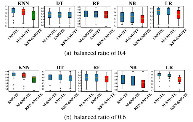
Fig. 13. The Scott-Knott ESD test ranking of the performance of SMOTE, M-SMOTE, and KFN-SMOTE in terms of pd on the five classifiers across 30 datasets under different balanced ratio (blue>red>green). (For interpretation of the references to color in this figure legend, the reader is referred to the web version of this article.)
