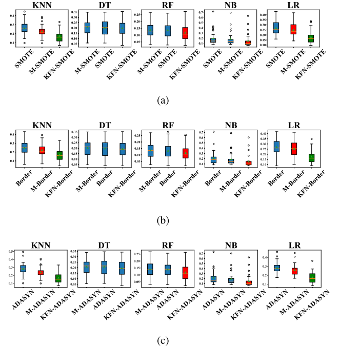
Fig. 9. The Scott-Knott ESD test ranking of the performances of SMOTE-based, M-SMOTE-based, and KFN-SMOTE-based techniques in terms of pf on the five classifiers across 30 datasets (blue>red>green). (For interpretation of the references to color in this figure legend, the reader is referred to the web version of this article.)
