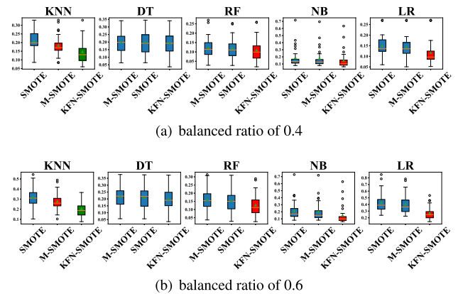
Fig. 14. The Scott-Knott ESD test ranking of the performance of SMOTE, M-SMOTE, and KFN-SMOTE in terms of pf on the five classifiers across 30 datasets under different balanced ratio (blue>red>green). (For interpretation of the references to color in this figure legend, the reader is referred to the web version of this article.)
