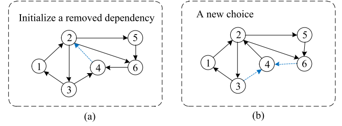
Fig. 5. An example of cycle breaking. A new choice (removing edges 3 \rightarrow 4 and 6 \rightarrow 4 ) with lower stubbing cost replaces the initially removed edge 4 \rightarrow 2 .
