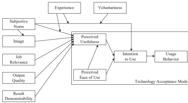
Fig. 3. TAM2 Model
