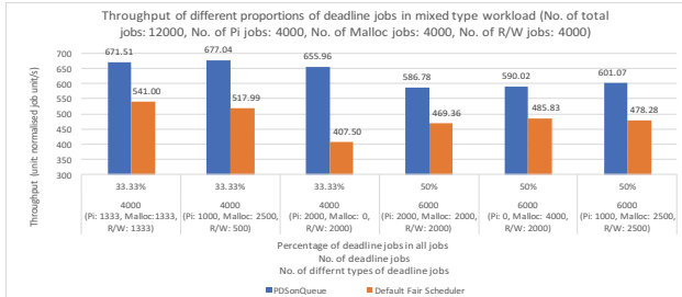
Fig. 3. Throughput on a mixed workload
