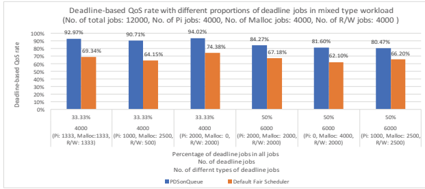
Fig. 2. Deadline-based QoS rate on a mixed workload
