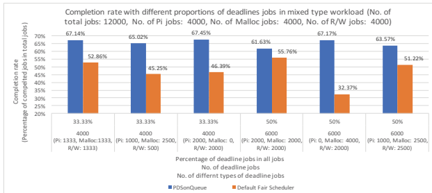
Fig. 4. Completion rate on a mixed workload
