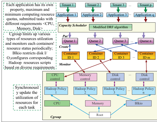
Figure 2. Our proposed Dominant Resource Fairness allocation algorithm
