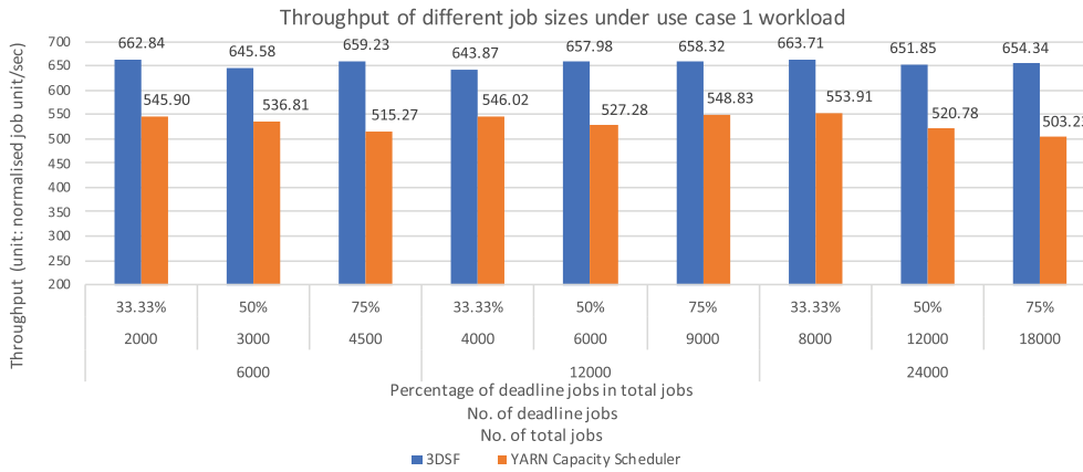
FIGURE 20 Throughput on the workload running case 1
