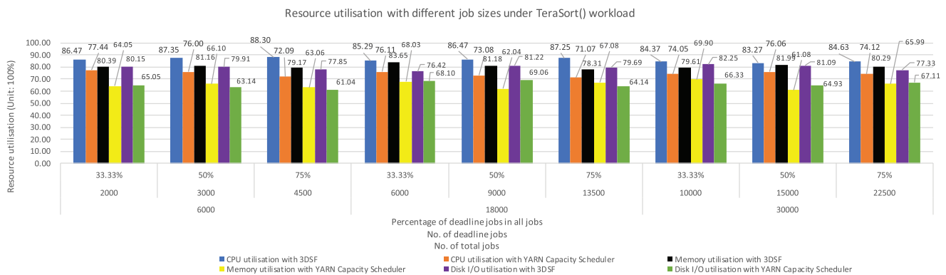
FIGURE 13 Resource utilization on TeraSort() jobs workload
