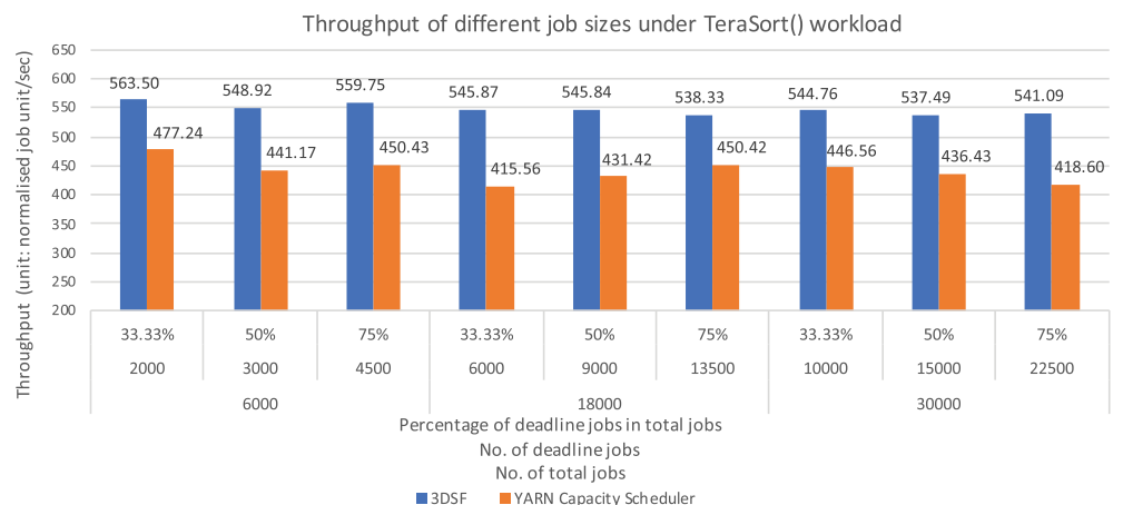
FIGURE 10 Throughput on TeraSort() jobs workload
