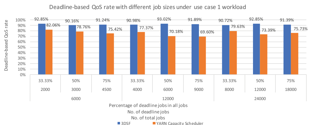
FIGURE 19 Deadline-based QoS rate on the workload of case 1
