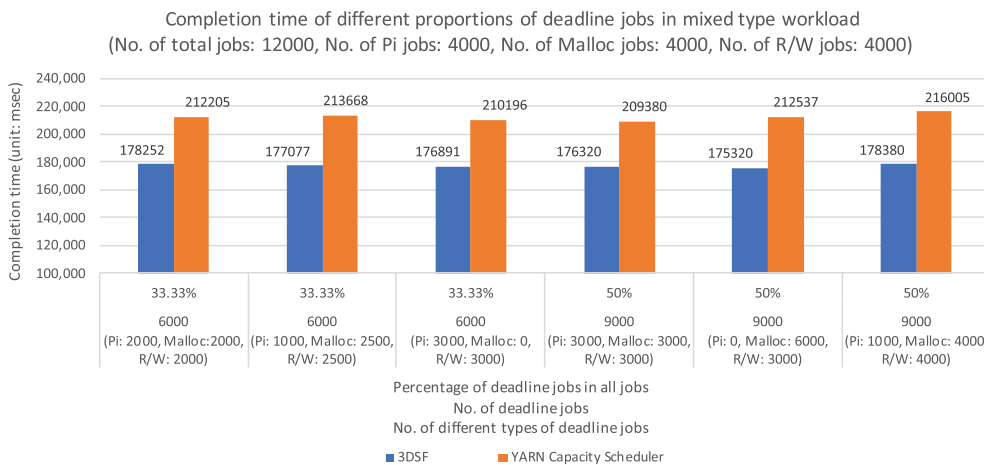
FIGURE 17 Completion time on a mixed workload
