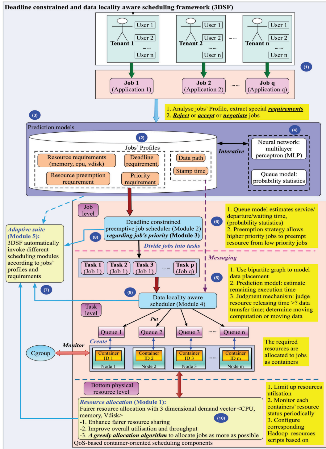
FIGURE 8 Architecture of 3DSF
