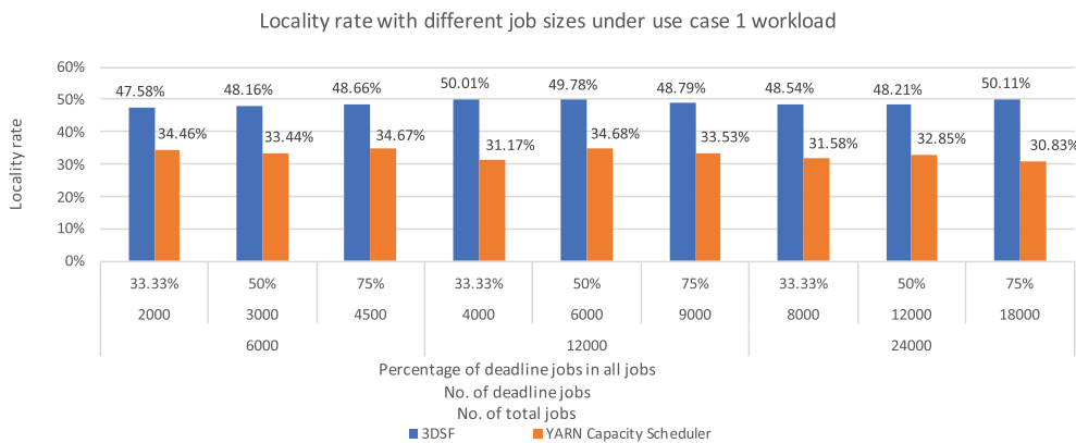
FIGURE 21 Locality rate on the workload running case 1
