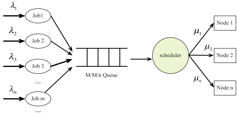
FIGURE 5 M/M/n queuing model for job performing in cloud computing
