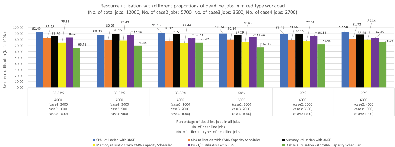
FIGURE 28 Resource utilization on a mixed cases workload
