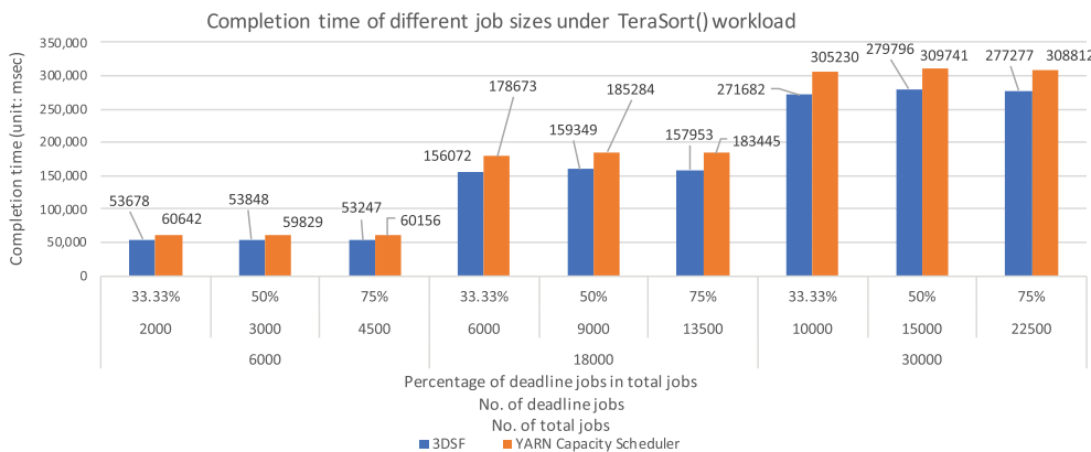
FIGURE 12 Completion time on TeraSort() jobs workload
