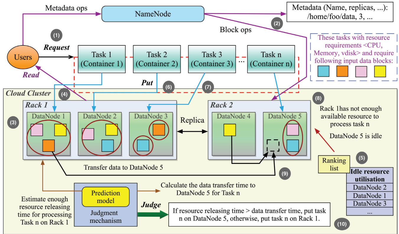
FIGURE 4 DLAforBT scheduler architecture: moving computation or moving data?
