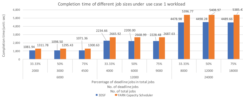
FIGURE 22 Completion time on the workload running case 1
