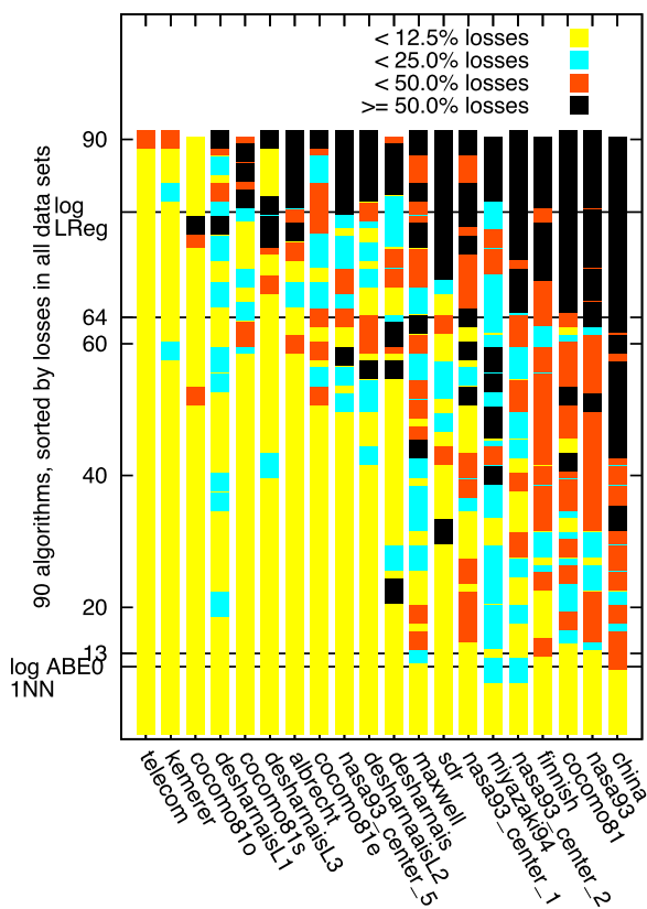
Fig. 7 Number of losses seen in 90 predictors and 20 datasets expressed as a percentage of the maximum losses possible for one predictor in one dataset (so 100\% = 89 \text{ comparison} \times 7 \text{ error measures} = 623 ; 50\% = 311 ; 25\% = 156 ; 12.5\% = 78 ). The predictors on the y-axis are sorted according to Fig. 4
