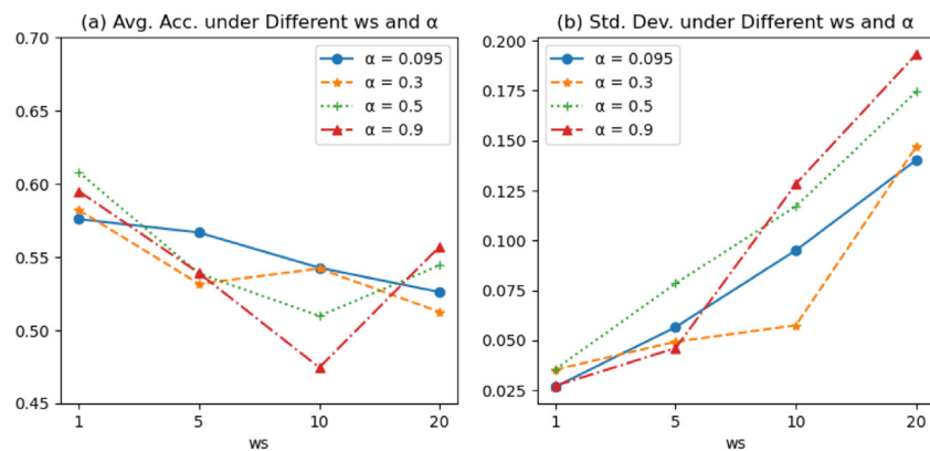
Fig. 4. The average accuracy and the standard deviation comparison among different ws and \alpha .
