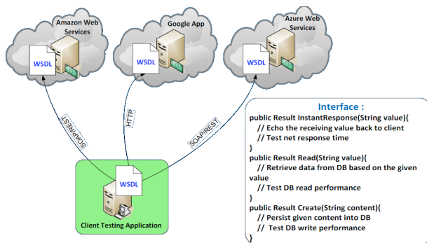
Figure 3. Contract-First Web Service based client
