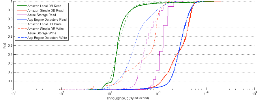
Figure 7. CDF of High Stress Database Read/Write throughput on Cloud databases (1KB data)
