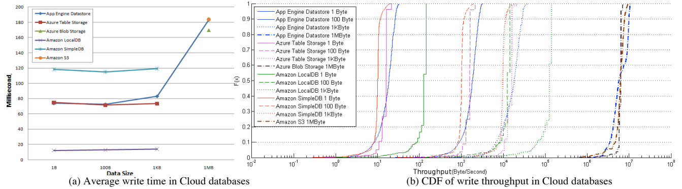
Figure 6. Low Stress Database Write (1B, 100B, 1KB and 1MB data)
