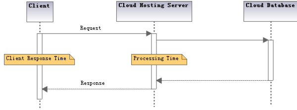
Figure 1. Time measurement terminologies
