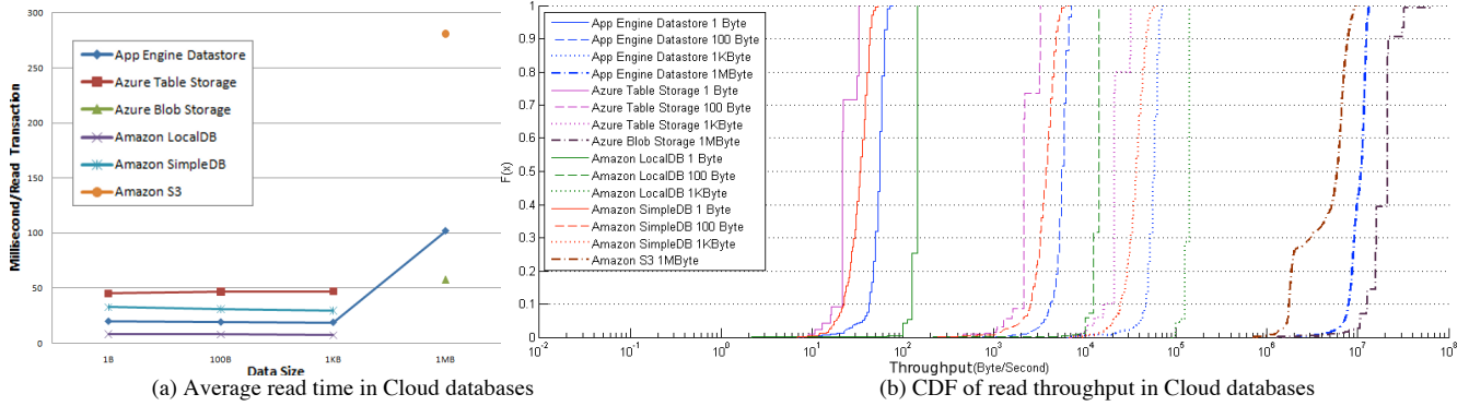
Figure 5. Low Stress Database Read (1B, 100B, 1KB and 1MB data)
